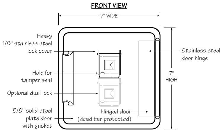
4500 Surface Mount
