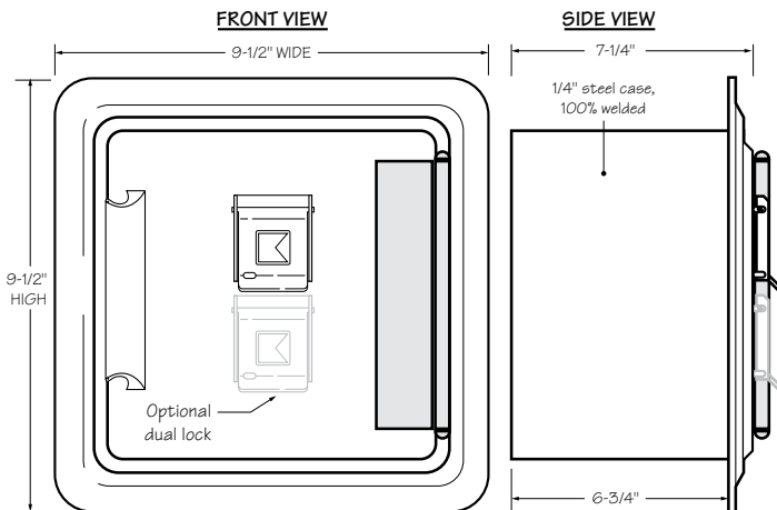
4500 Recessed Mount
